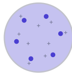
Thomson (1897)
