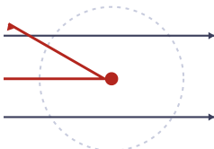
Rutherford (1911)
